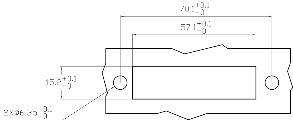
PANEL PREPARATION
