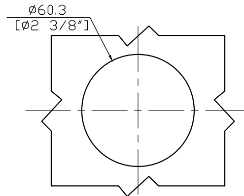
PANEL PREPARATION
