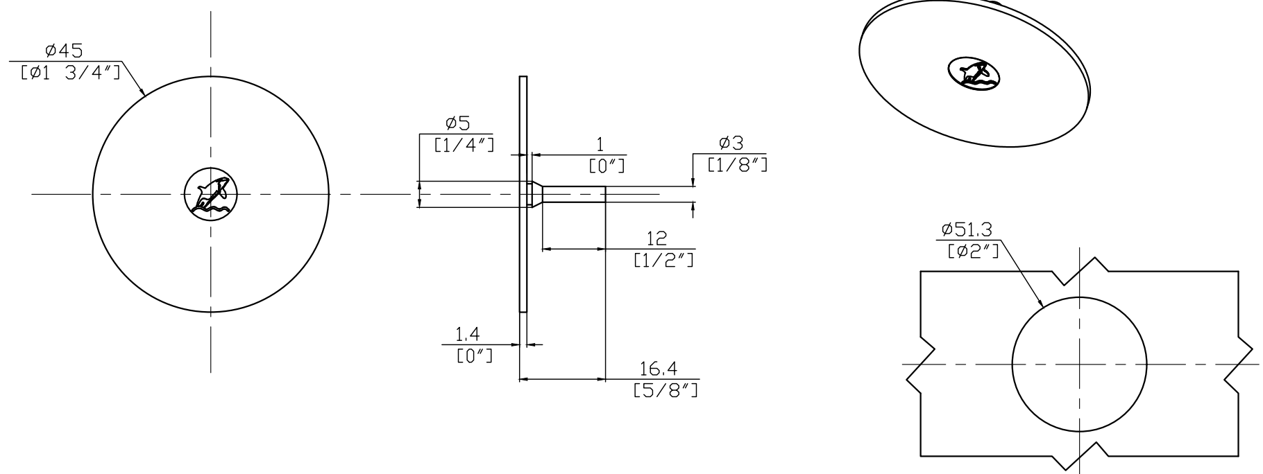
PANEL PREPARATION
