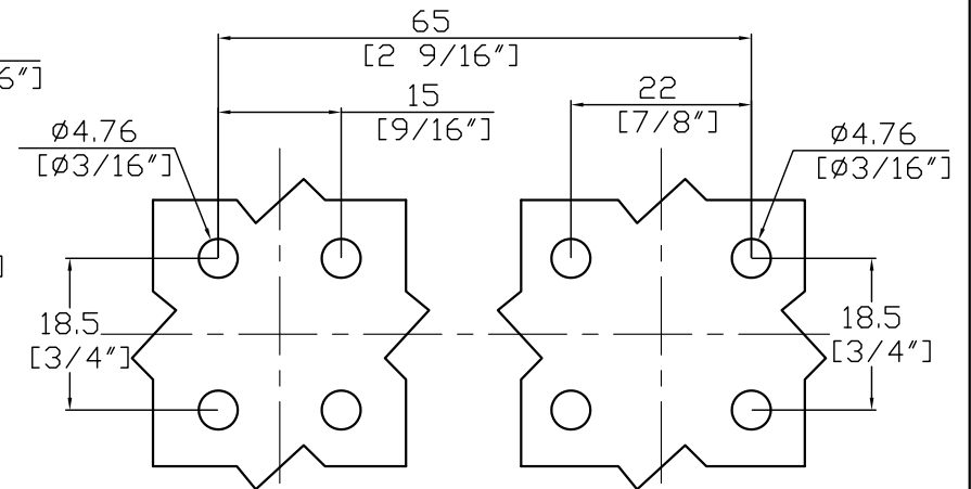
PANEL PREPARATION
