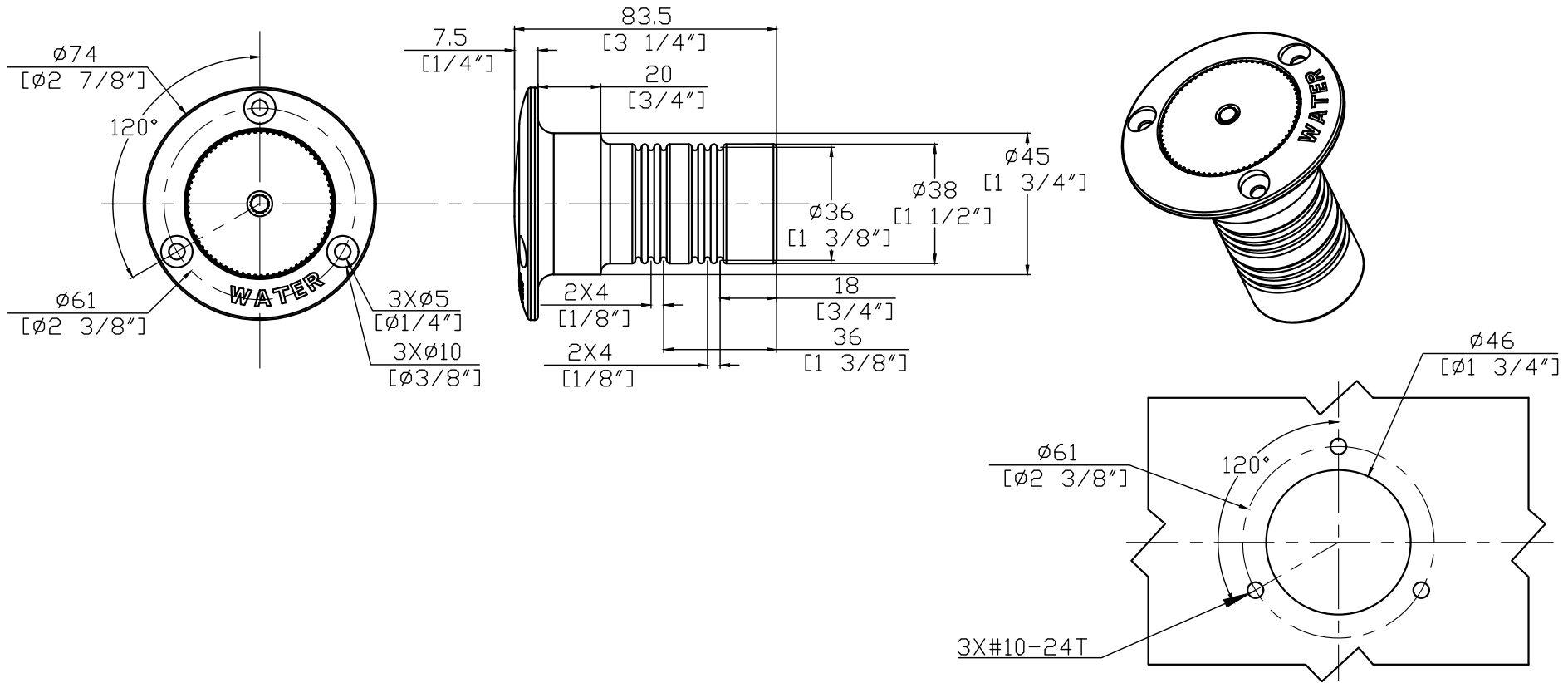
PANEL PREPARATION
